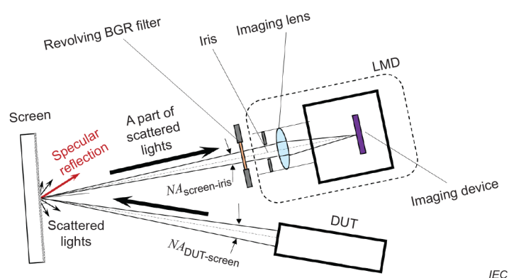
Figure 29 – Example of measurement geometries for colour speckle using an LMD with BGR filters
