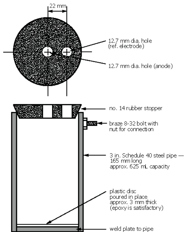
FIG. 1 Detail of Test Pot
