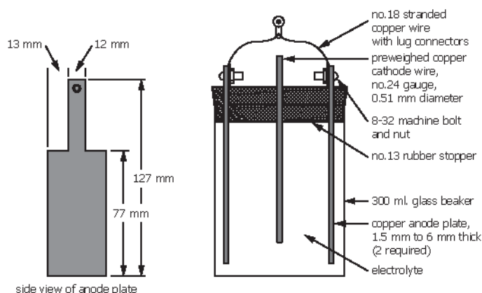
FIG. 2 Copper Coulometer
