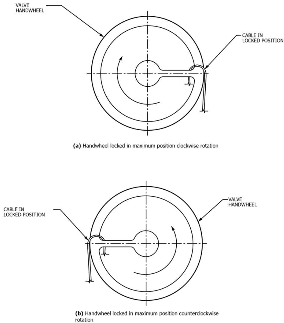
FIG. 2 Miscellaneous Type I Details
