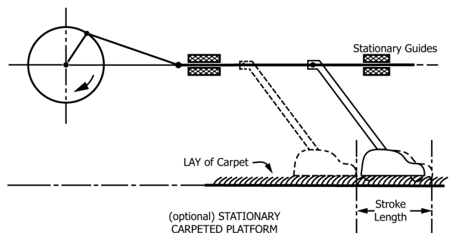
FIG. 1 Test Fixture
