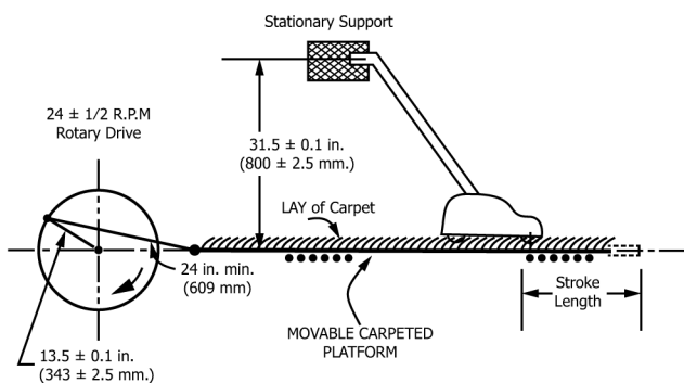
FIG. 1 Test Fixture
