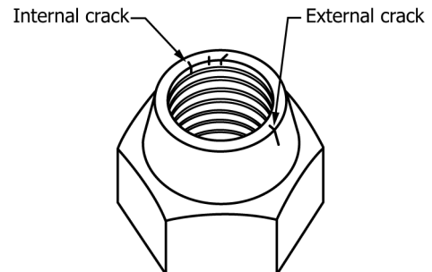
FIG. 3 Typical Locking Element Cracks in Prevailing-Torque Nuts
