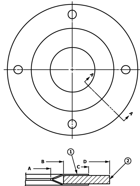
FIG. 2 Split Design (Full Face)
