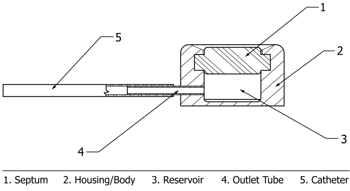
FIG. 2 Example of an Implantable Port (section)
