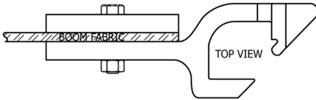
FIG. 1 Connector Orientation
