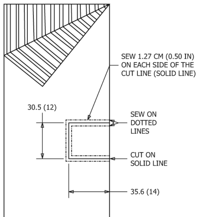
FIG. 1 Test Specimen
