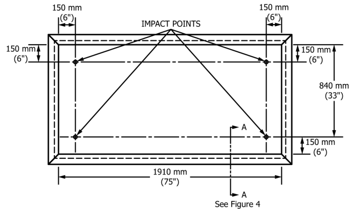
FIG. 1 Frame Dimensions and Location of Test Impact Points
