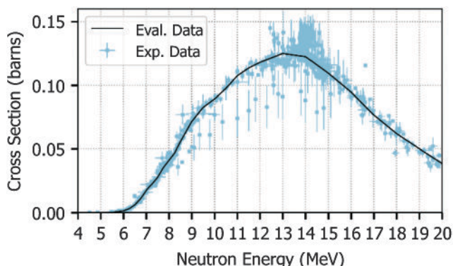
FIG. 1 ^{27}\text{Al}(n,\alpha)^{24}\text{Na} Cross Section, from IRDF-II Library, with EXFOR Experimental Data
