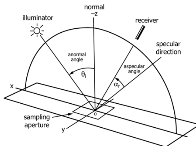
FIG. 1 Uniplanar Configuration
