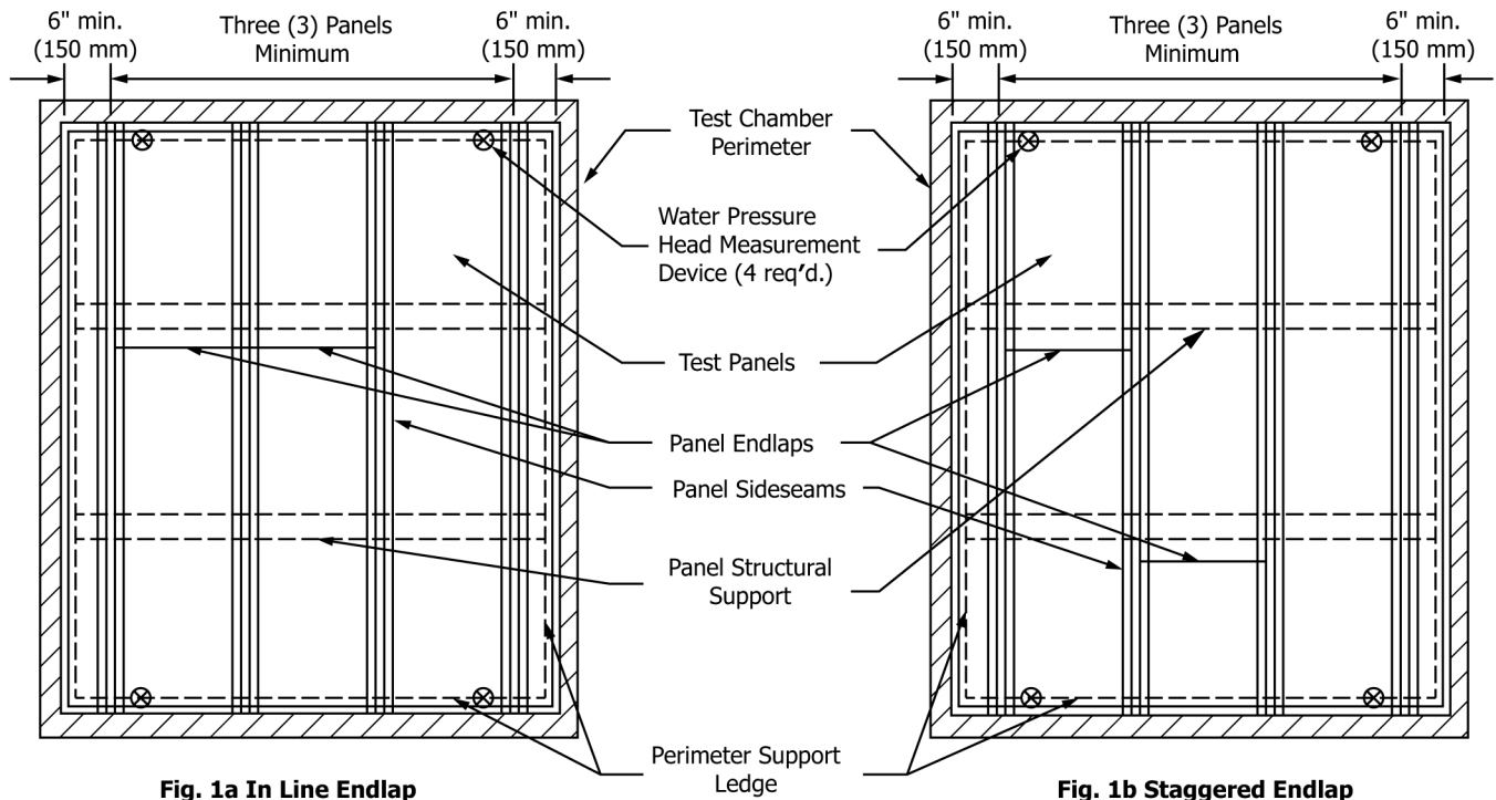
FIG. 1 Plan of Typical Three-Span Test Specimen Mounted in Chamber
