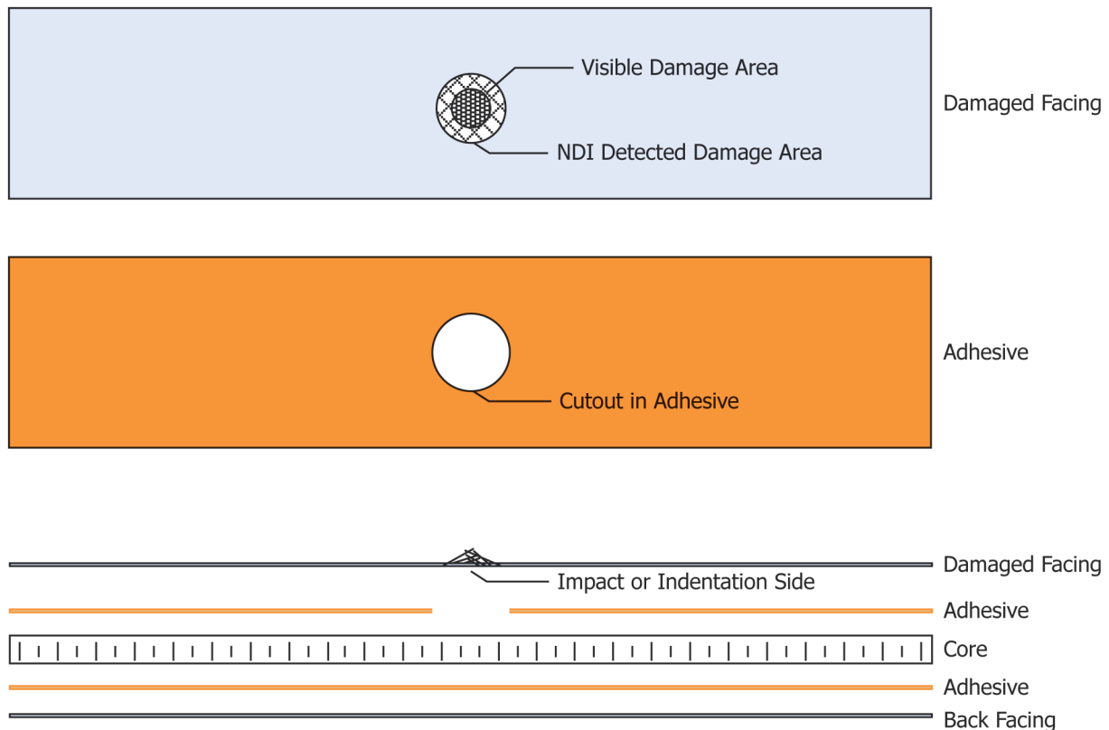
FIG. 1 Sandwich Specimen Assembly
