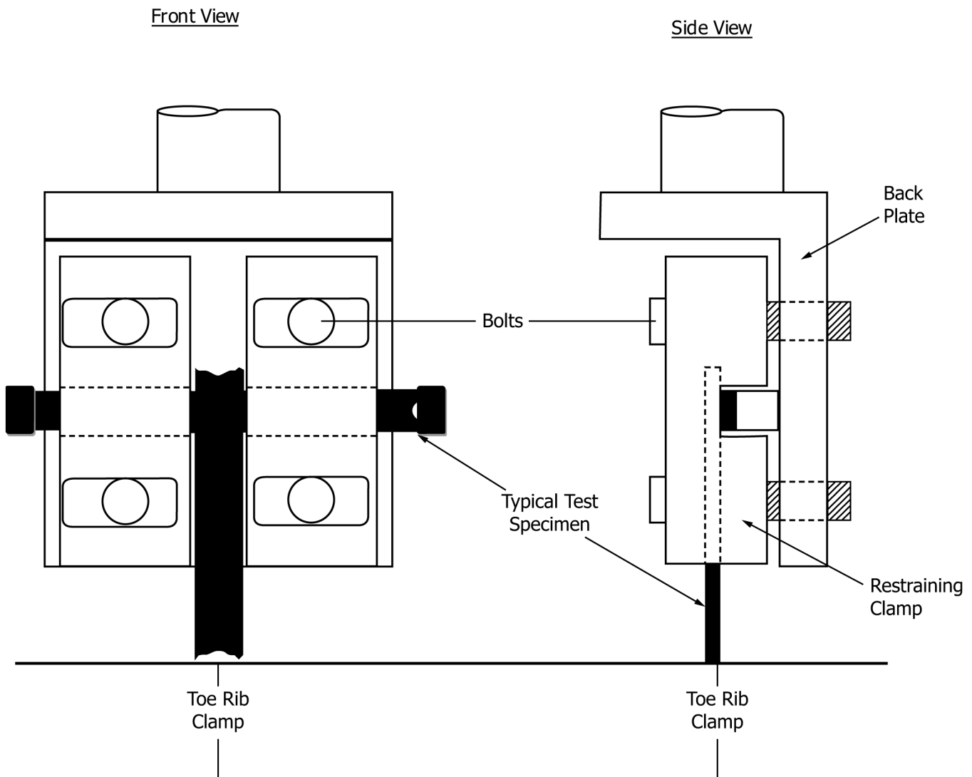
FIG. 1 Typical Junction Strength Test Specimen Test Setup (rotation is not constrained per 6.3)
