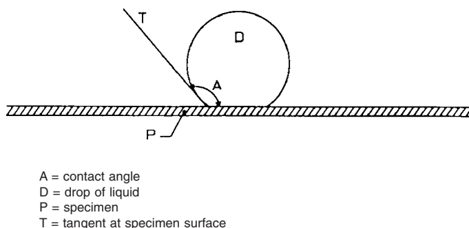
FIG. 1 Measuring Angle of Contact
