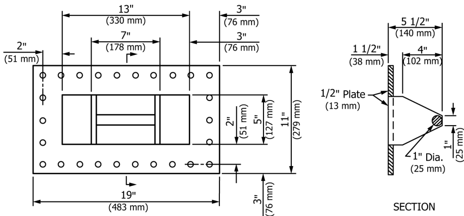
FIG. 2 Clamping Bracket
