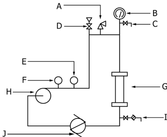
FIG. 2 High Temperature Test Equipment
