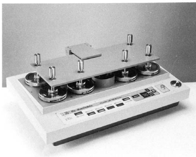
FIG. 1 Martindale Tester
