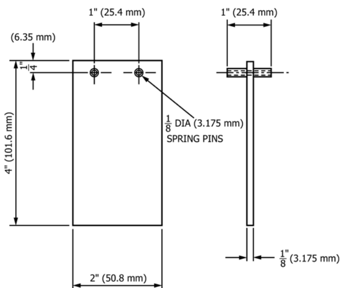
FIG. 1 Aluminum Plate
