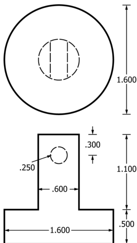
FIG. 1 Loading Fixture
