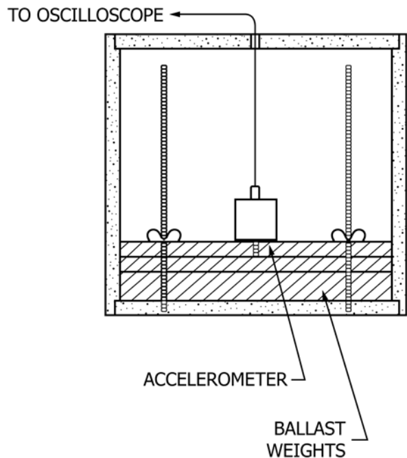
FIG. 2 Test Block
