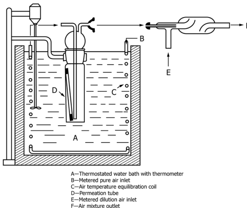
FIG. 1 Optional System for Laboratory Use of a Permeation Tube
