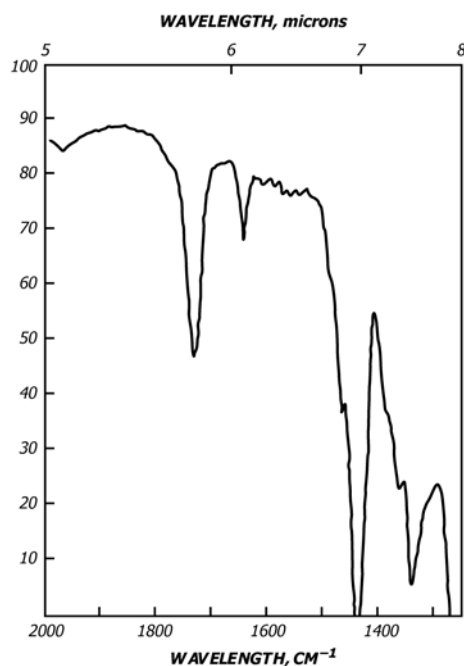
FIG. 1 Calibration Curve, 1 % Plasticizer in PVC Resin at 5.8 µm
