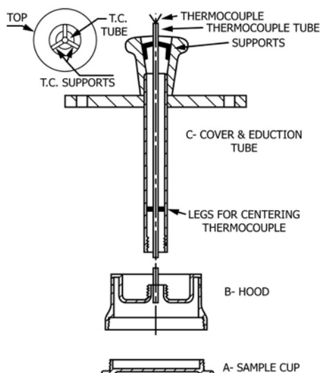
FIG. 1 Thermocouple Arrangement
