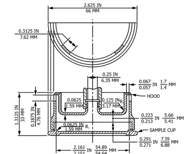
SECTION OF GREASE SAMPLE CUP ALL DIMENSIONS \pm 0.0156 in. ( \pm 0.4 mm) UNLESS OTHERWISE SPECIFIED
