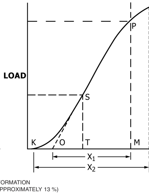
FIG. 1 b Compressive Strength (See 3.1.5 and Section 9)
