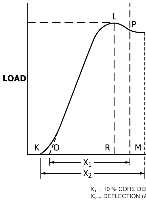
FIG. 1 a Compressive Strength (See 3.1.5 and Section 9)
