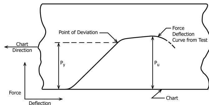
FIG. 2 Force Deflection Chart
