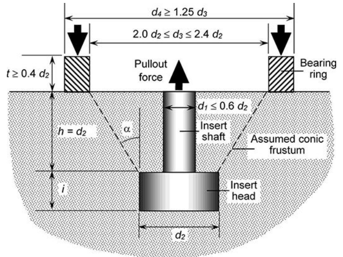
FIG. 1 Schematic Cross Sectional View of Cast-in-Place Pullout Test
