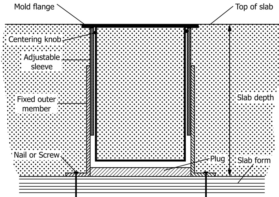
FIG. 1 Schematic of Cast-in-Place Cylinder Mold Assembly
