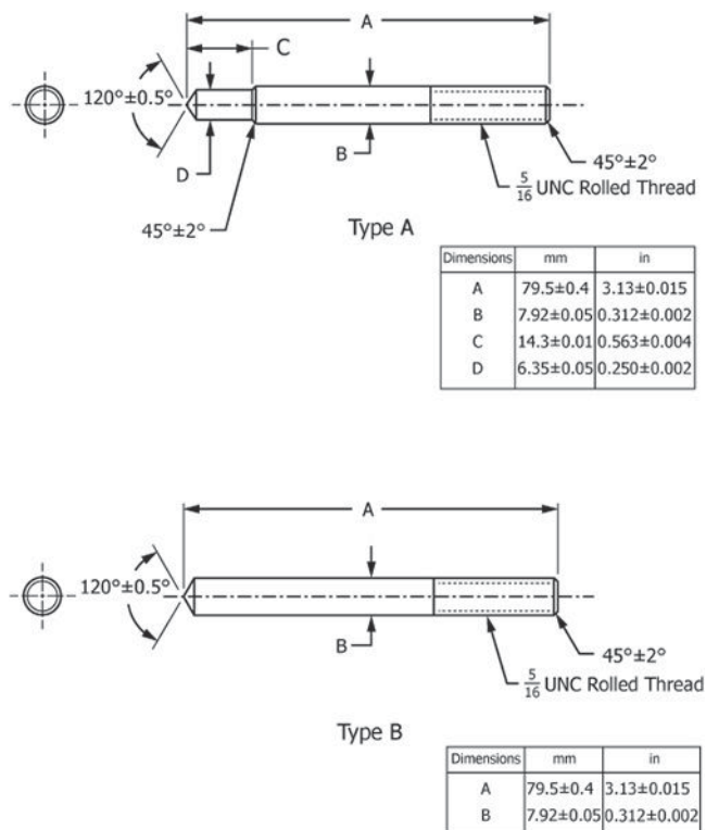
FIG. 1 Dimensions of Probes
