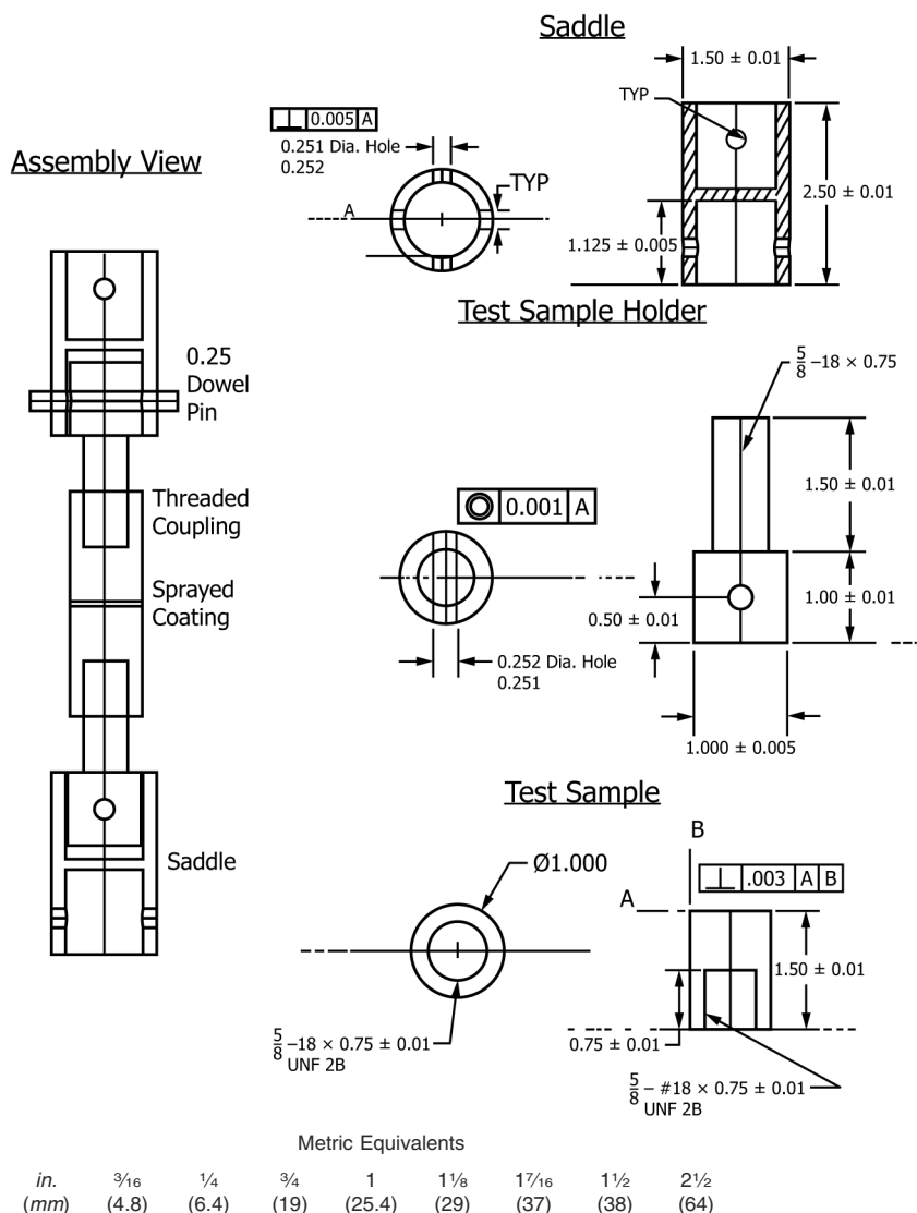
FIG. 1 Self-Aligning Device
