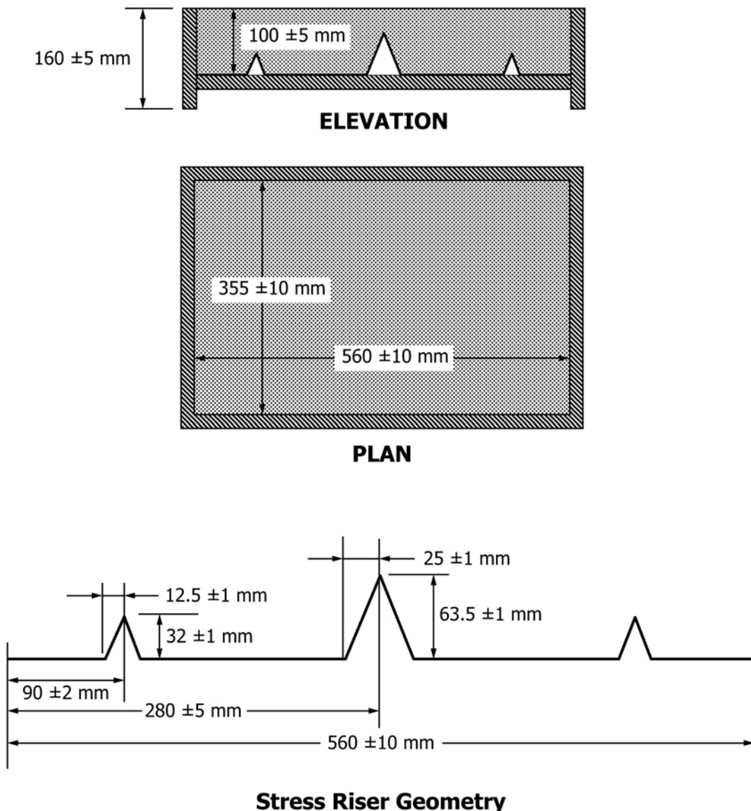
FIG. 1 Specimen and Stress Riser Geometry (4, 3)
