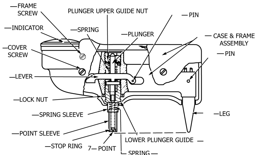
FIG. 1 Diagram of Typical Barcol Impressor Arrangement
