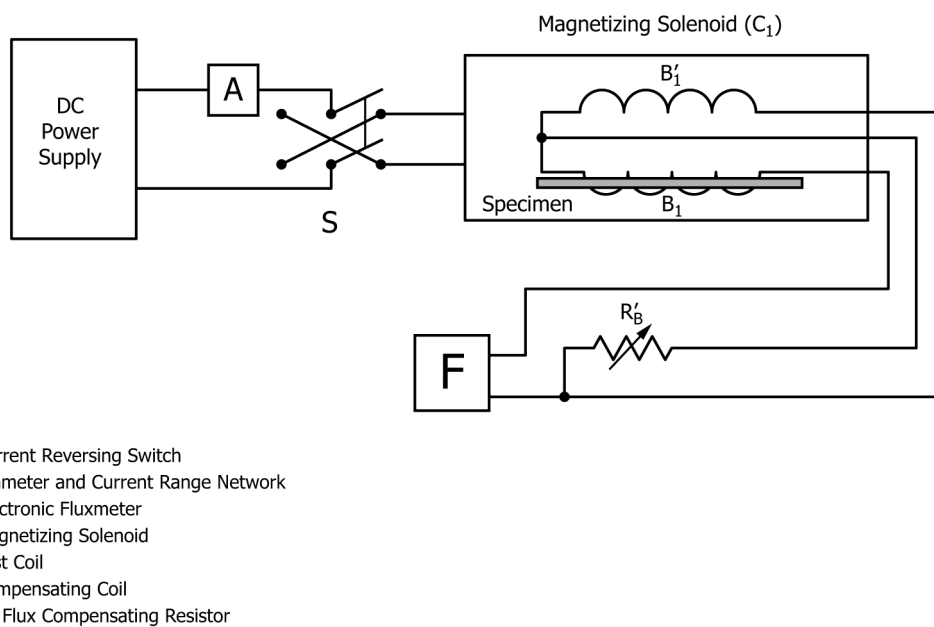
FIG. 1 Circuit Diagram for Method No. 1
